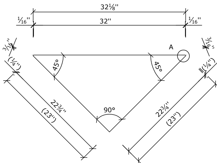
top view ( 1 : 10 )
