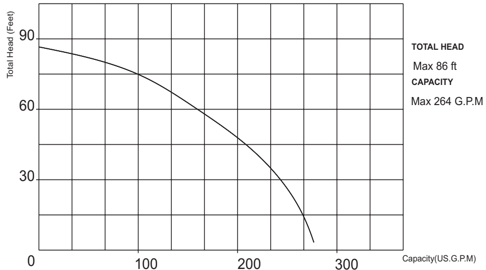
Performance Curve
